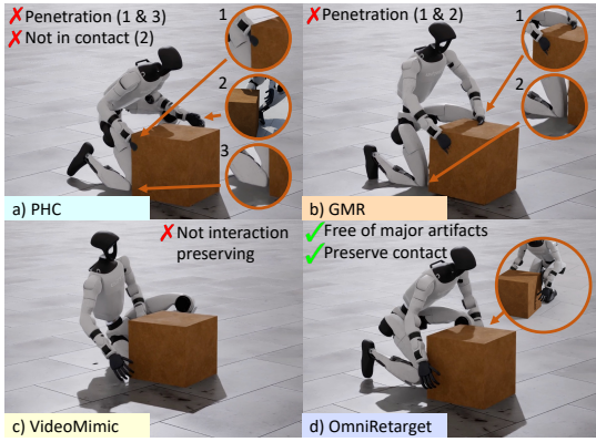
Fig. 6: Artifacts resulting from the retargeting baselines.
