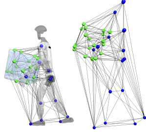
Fig. 8: The actual target (left) and source (right) interaction meshes used for optimization.
