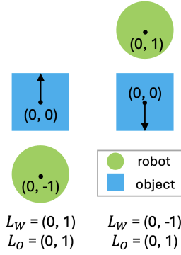
Fig. 7: The Laplacian coordinate should stay the same when the object rotates 180^\circ .
